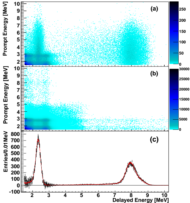
FIG. 1: (color online) (a) The prompt vs. delayed energy of double coincidence events with a maximum 50 cm vertex separation for all far-hall ADs, (b) the accidental background sample (ABS) events and (c) the delayed energy distribution after subtracting the accidentally coincident background for the far hall (black) and the near halls (red), where the total near site spectrum was normalized to the area of the far site spectrum.
